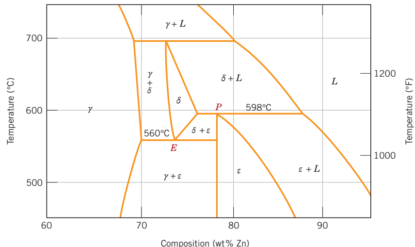
Figure 9.21 A region of the copper–zinc phase diagram that has been enlarged to show eutectoid and peritectic points, labeled E (560°C, 74 wt% Zn) and P (598°C, 78.6 wt% Zn), respectively. [Adapted from Binary Alloy Phase Diagrams , Vol. 2, 2nd edition, T. B. Massalski (Editor-in-Chief), 1990. Reprinted by permission of ASM International, Materials Park, OH.]
