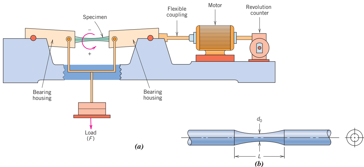
Figure 8.19 For rotating-bending fatigue tests, schematic diagrams of (a) a testing apparatus, and (b) a test specimen.
