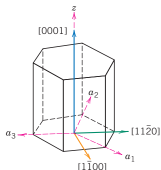
Figure 3.9 For the hexagonal crystal system, the [0001] , [1100] , and [11\bar{2}0] directions.
