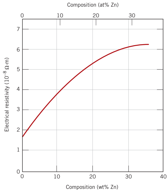
Figure 18.37 Room-temperature electrical resistivity versus composition for copper–zinc alloys.
