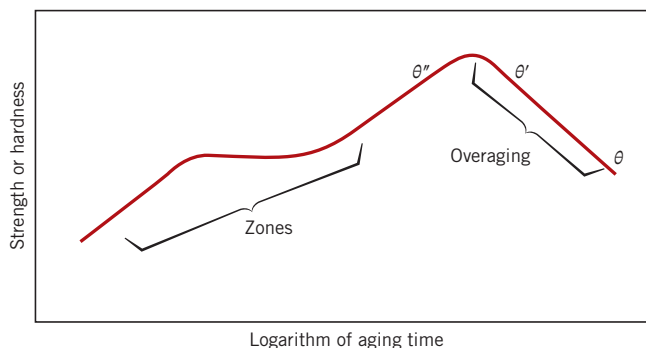
Figure 11.28 Schematic diagram showing strength and hardness as a function of the logarithm of aging time at constant temperature during the precipitation heat treatment.
